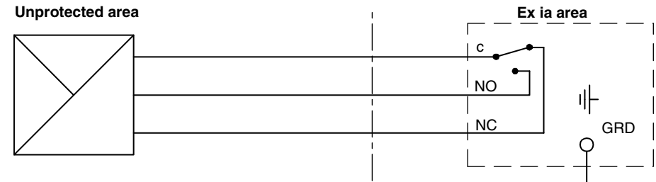
Fig. 7: Operation of pressure switches in intrinsically safe areas
